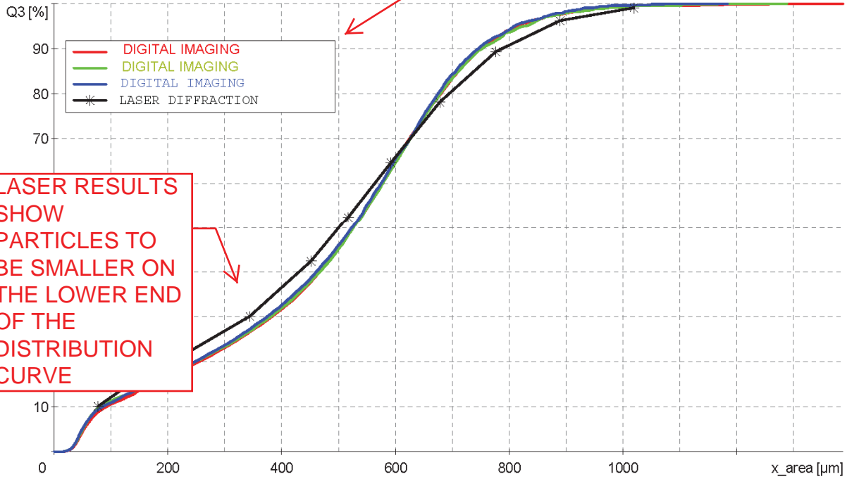
COFFEE GRINDS COMPARING LASER DIFFRACTION TO DIGITAL IMAGING
