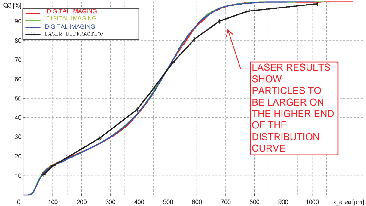
COFFEE GRINDS LASER DIFFRACTION VS DIGITAL IMAGE ANALYSIS
